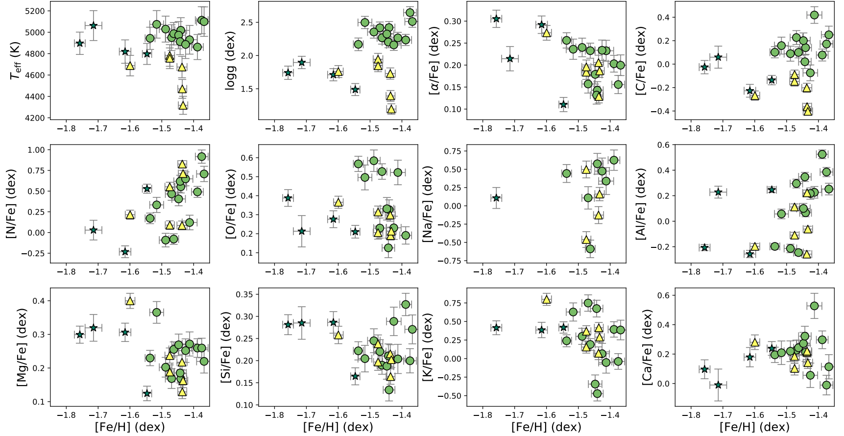
Figure 2.4: T_{\text{eff}} , \log g , and [X/\text{Fe}] for surface parameters and abundances in Table 5.1. It can be noticed from the Figure, for a given metallicity there is a large spread for certain elements ( [\text{N}/\text{Fe}] , [\text{C}/\text{Fe}] , [\text{Na}/\text{Fe}] , and [\text{Al}/\text{Fe}] ). The AGB group (green stars) and one uRGB star (yellow triangle) is completely offset from the global trend. This spread in [\text{Fe}/\text{H}] values was the main reason which led us to consider and publish the median over the mean values for the elemental abundances.
