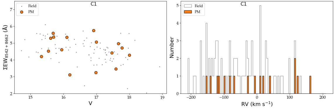
Figure 5.7: (Left panel): EW of the two most prominent lines in the CaT versus the V magnitude for C1. Circular orange symbols represent the PM-selected stars matched with the MUSE extracted spectra and grey points represent the field stars present in the cube. Note that no clear relation between the EW and V-magnitude is observed, contrary to the expected GC behaviour. (Right panel): RV histogram of all the sources in the MUSE cube colour-coded by a selection procedure: orange for the PM and grey for the field stars in the FoV. No RV peak is seen within the 16 matched Gaia PM-selected stars.
