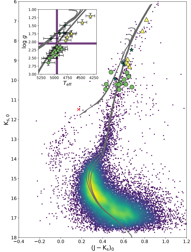
Figure 2.2: Dereddened (J-K_s) \times K_s color-magnitude diagram of NGC 6544 members from VVV ( K_s \gtrsim 11 mag, Contreras Ramos et al., 2017) and 2MASS ( K_s \lesssim 11 mag Skrutskie et al., 2006; Valenti et al., 2007). As mentioned in the text, different symbols were used to differentiate within stellar stages. Circles, triangles, and stars were used to highlight different evolutionary stages based on their positions on the T_{\text{eff}}\text{-log } g diagram (see section 2.1.3 for definitions). Subsequent figures will use the same markers. The RR Lyrae star analysed in section 2.1.4 is marked with a cross. ( Inset ): T_{\text{eff}}\text{-log } g diagram of the 23 APOGEE cluster candidates together with the same three PARSEC isochrones. All of them for the same metallicity and \alpha -enhancement values of the cluster, for ages of 10, 12 and 14 Gyr. The RGB bump is marked at the intersection of the two shaded areas.
