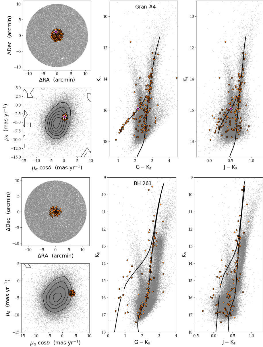
Figure 4.4: ( Upper four panels ): Spatial distribution, VPD, and near-IR-optical ( G - K_s and J - K_s ) CMD for the Gran 4 GC with identical panel distribution as in Figure 4.3. A PARSEC isochrone of 12 Gyr and [\text{Fe}/\text{H}] \sim -2.4 dex is presented as a reference. The cluster member RR Lyrae star is marked with a star in all the panels. ( Lower four panels ): Same as in the upper panels, but for BH 261. Note that we draw the AGB phase in the CMD, since the possible association of some stars to that stage, as two parallel sequences can be appreciated in both near-IR-optical CMDs at K_s \geq 13 mag. The selected isochrone is a composition of a PGPUC (SGB, RGB and HB) and a PARSEC (AGB) models as it is described in Sec. 4.1.8. Both isochrones are for a metallicity of -2.4 dex and shifted by a distance modulus of 14.80 mag.
