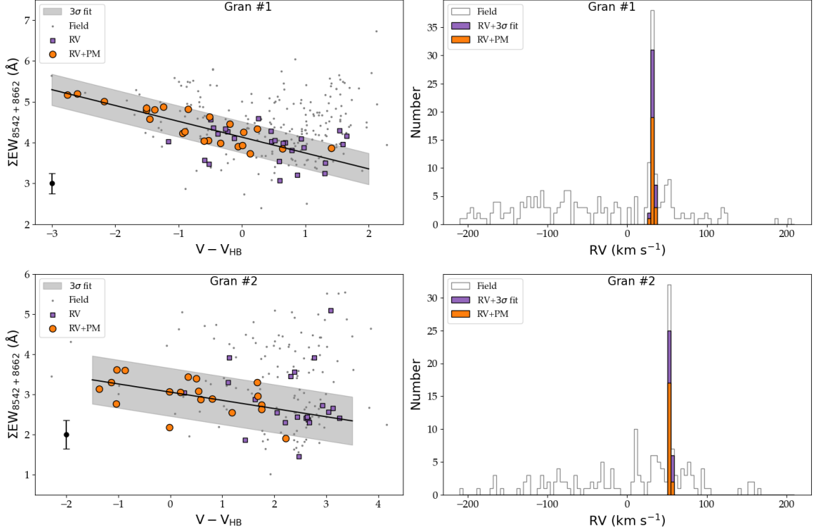
Figure 4.9: (Upper left panel): EW of the two most prominent lines in the CaT versus the V magnitude normalised to the HB level for the GC Gran 1. Circular orange symbols represent the PM-selected stars matched with the MUSE extracted spectra, purple squares show the stars selected by RV within 5 km s -1 from the cluster value, and grey points represent the field stars present in the cube. The error bars of the black point represent the mean EW error for the stars in the MUSE field. The line fitted to the PM-selected stars is also shown with a shaded area and is equivalent to 3 times the intercept uncertainty. (Upper right panel): RV histogram of all the sources in the MUSE cube colour-coded by a selection procedure: orange for the PM, purple of the stars with RV that lie within the shaded area, and grey for the field stars in the FoV. (Upper middle left and upper middle right panels): Same as in the upper panels but for Gran 2. (Lower middle left and lower middle right panels): Same as in the upper panels but for Gran 3. (Lower left and lower right panels): Same as in the upper panels but for Gran 5.
